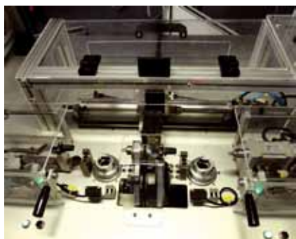
Check, marking & packaging station 功能检测设备
