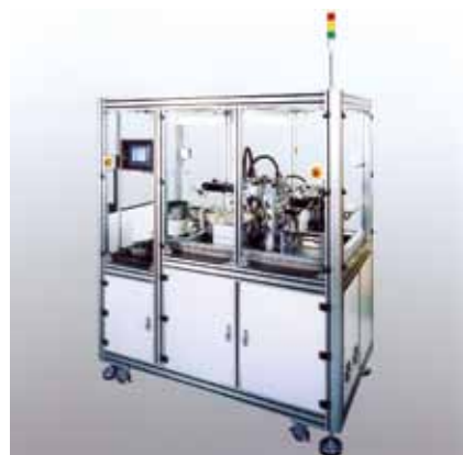
Disc Hub Assembly Assemble disc to hub with an adhesive tape in clean room environment and high precision.
